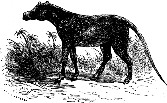
Fig. 15.—The Common Anoplotherium.
